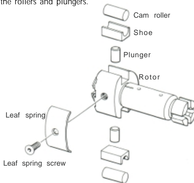
Fig. 4 — Rotor and plunger
