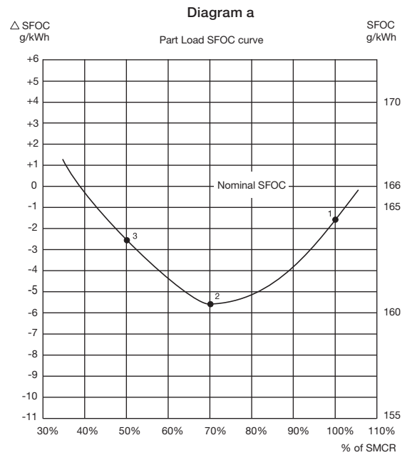
Fig. 2.10.01: Example of SFOC for derated 6G95ME-C9.5-TII with fixed pitch propeller and high efficiency turbocharger
