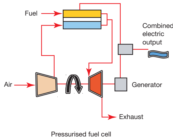
Figure 13: Solid oxide fuel cell schematic
