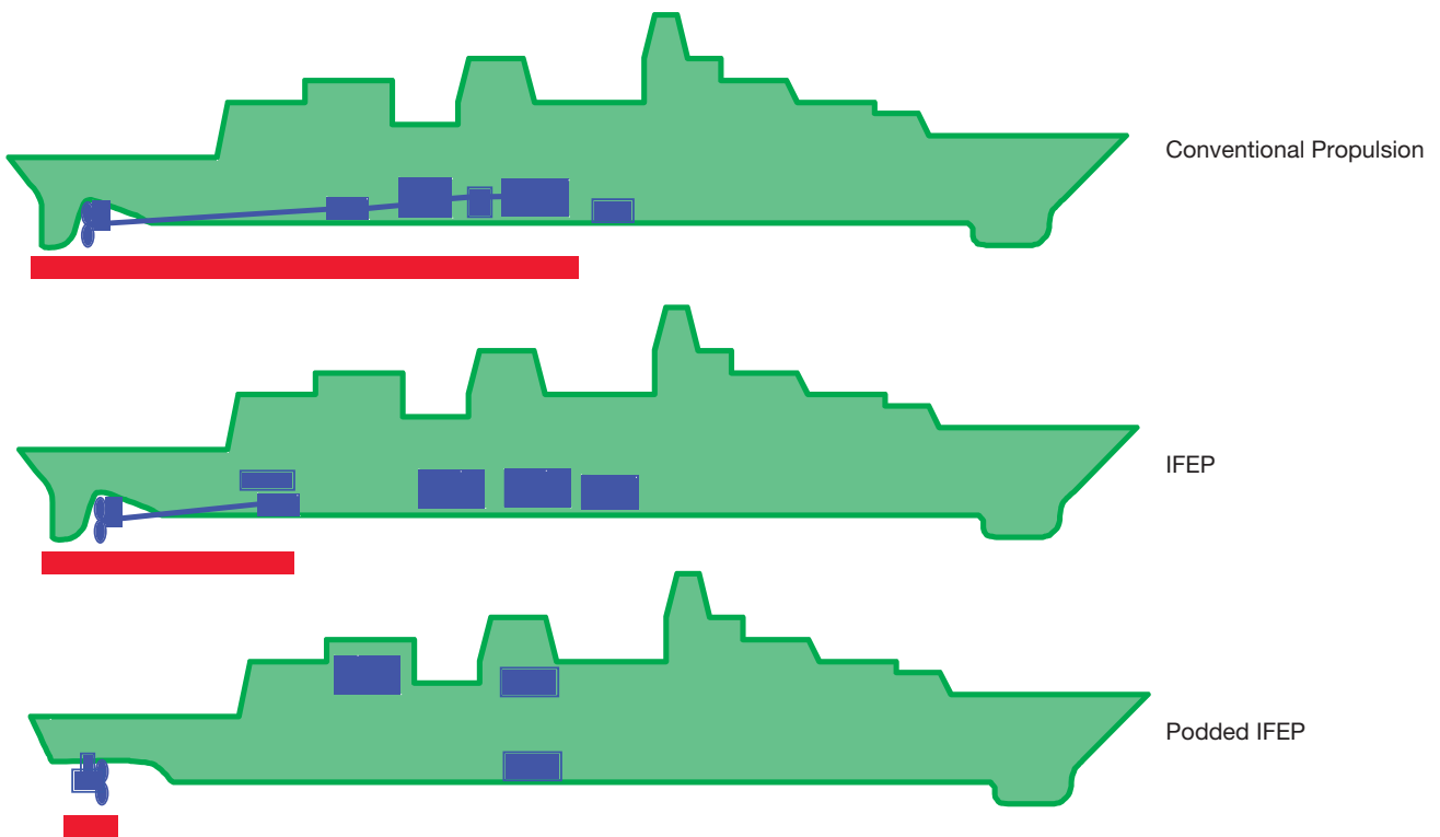
Figure 7: Layout of mechanical and electrical propulsion systems
