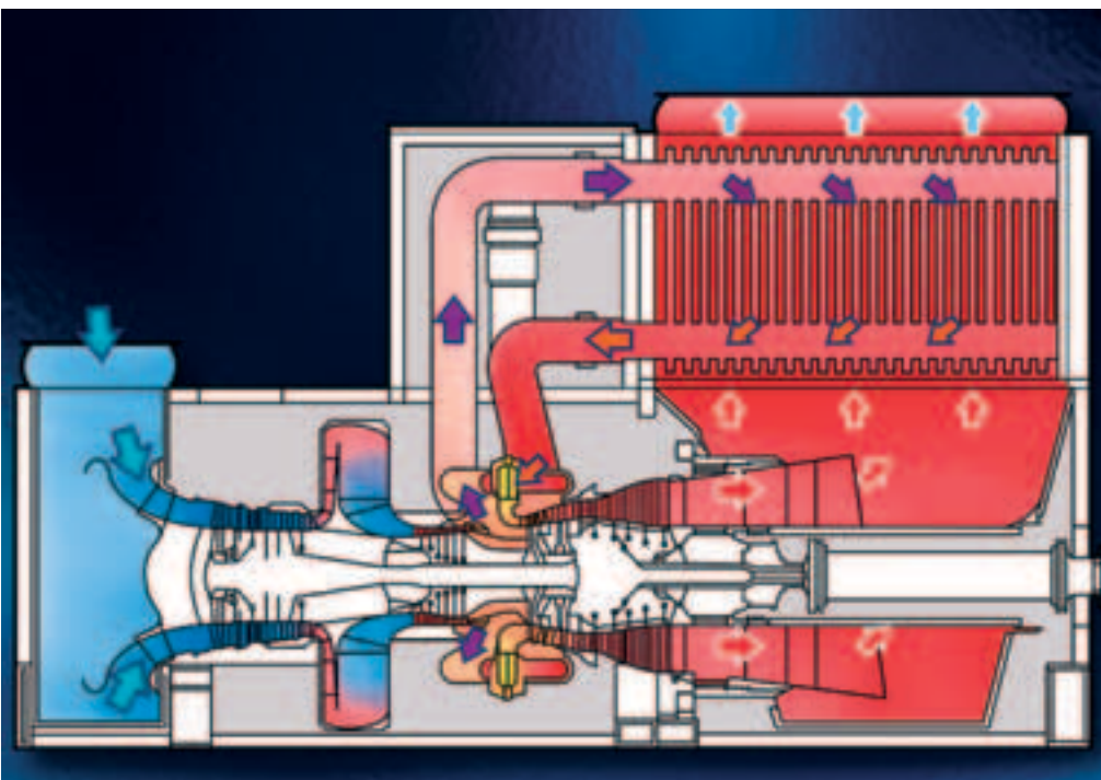
Figure 12: WR-21 gas turbine airflow diagram
