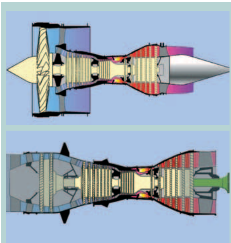
Figure 3: The Marine Trent and the Trent 800 (top) aeroengine
