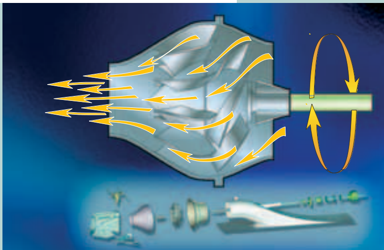
Figure 5: Construction and water flow through a waterjet
