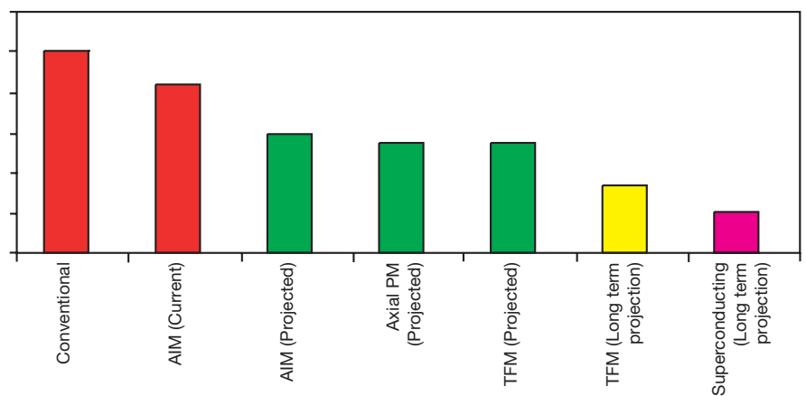
Figure 8: Comparative size of different propulsion motor technologies AIM – advanced induction motor PM – permanent magnet TFM – transverse flux motor
