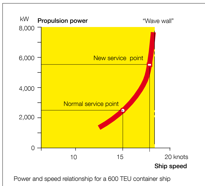
Fig. 5: The “wave wall” ship speed barrier
