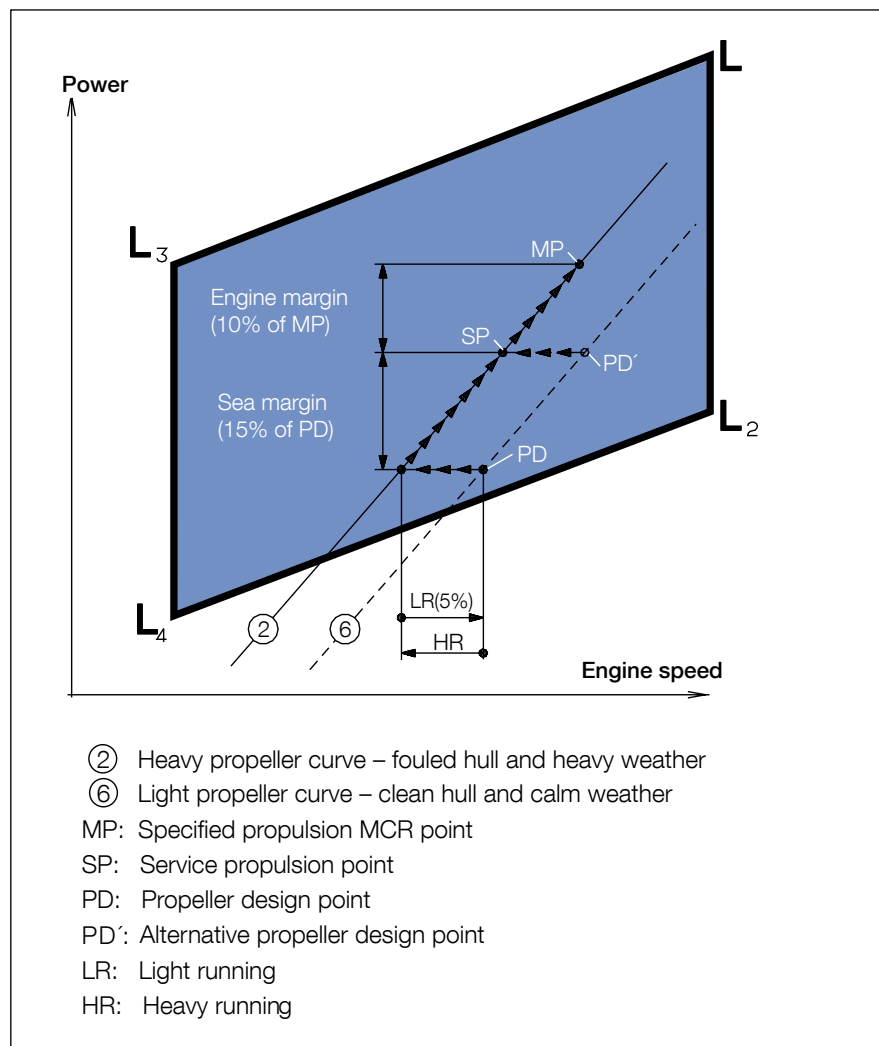
Fig. 17: Ship propulsion running points and engine layout
