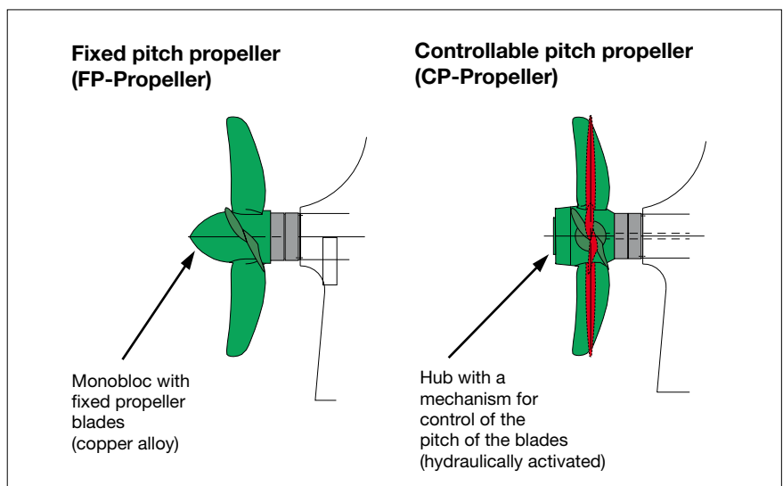
Fig. 7: Propeller types
