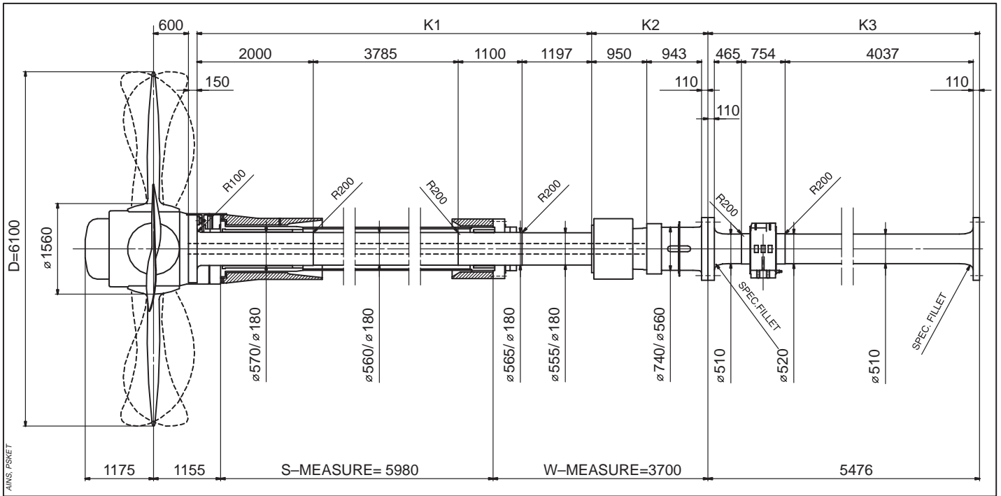
Fig 36: Propeller data for torsional vibration analysis
