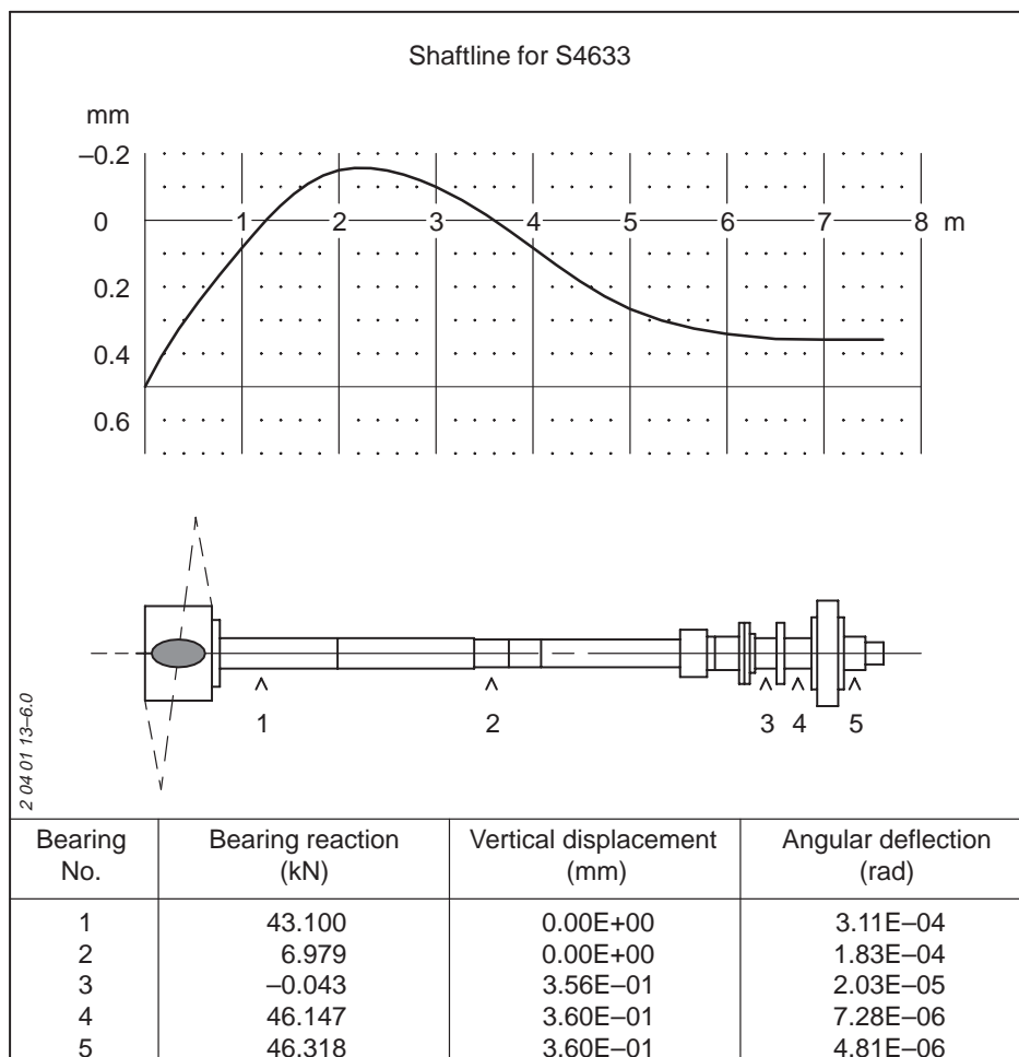
Fig 34: Calculated reactions and deflections in bearings
