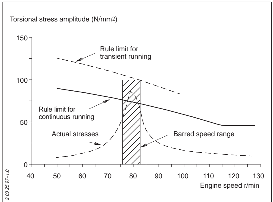
Fig 35: Torsional vibration calculation Bulk carrier project 6S50MC 8,580 kW/127 r/min Propeller shaft aft end (d= 460 mm/Ck = 0.55)
