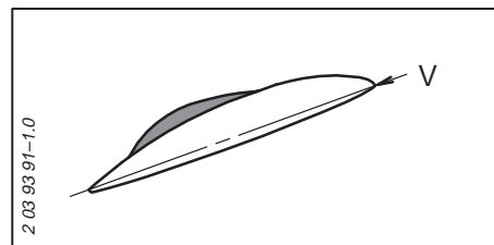
Fig 28: Suction side (bubble cavitation)
