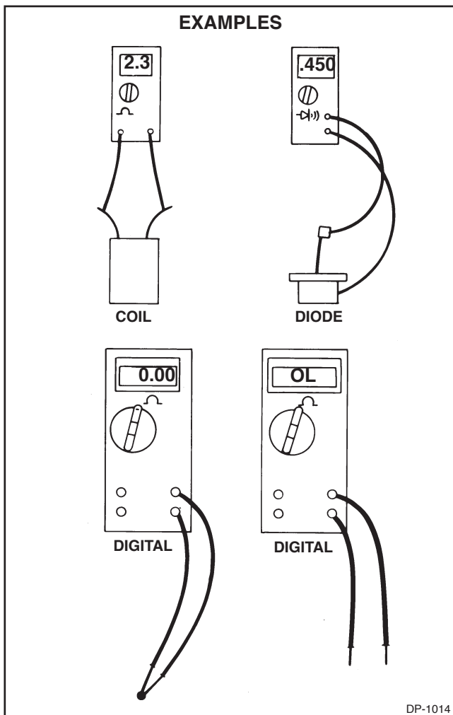
Figure 1-14. Digital Ohmmeter
