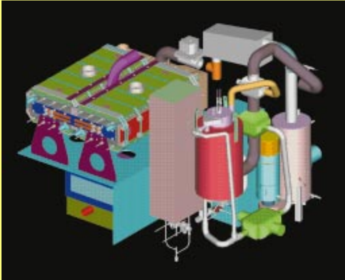
Computer model of 50kW fuel cell stack with reformer. (Courtesy: International Fuel Cells)
